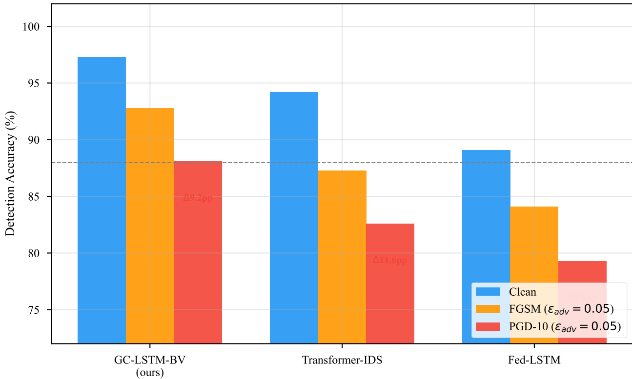
Adversarial Robustness Under White-Box Attacks
